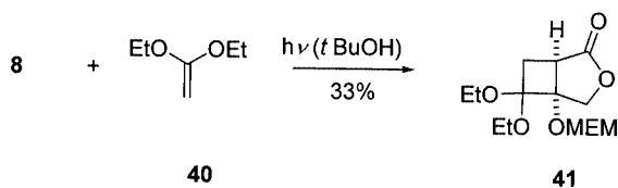
Scheme 12. Intermolecular cycloaddition of tetronate 8 and ketene diethyl acetal 40
