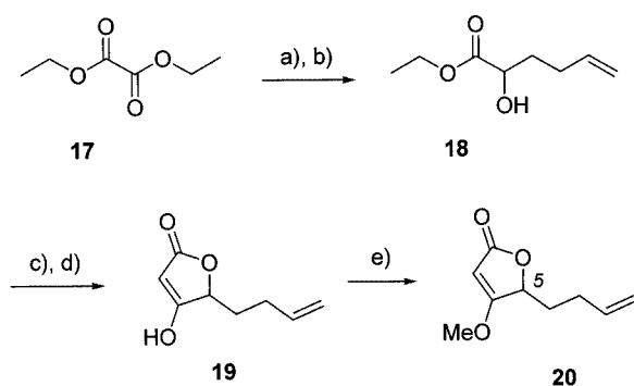
Scheme 4. Preparation of the C5-substituted methyl tetronate 20 from diethyl oxalate ( 17 ): a) \text{C}_4\text{H}_7\text{MgBr} in \text{Et}_2\text{O} , 83% b) \text{Na}(\text{CN})\text{BH}_3 in \text{EtOH}/\text{H}_2\text{O}/\text{HOAc} , 7:3:1, 80% c) \text{Ac}_2\text{O} in py, 83% d) LiHMDS in THF, 84% e) MeOH, \text{PPh}_3 , DIAD in THF, 94%
