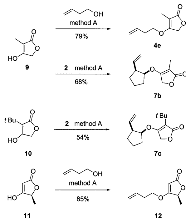
Scheme 2. Preparation of photocycloaddition precursors incorporating substituted tetronic acids 9–11
