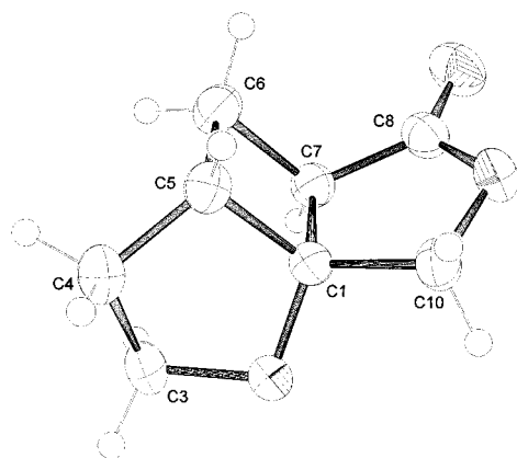
Figure 2. A molecule of 2,9-dioxatricyclo[5.3.0.0 1,5 ]decane ( 21 ) in the crystal
