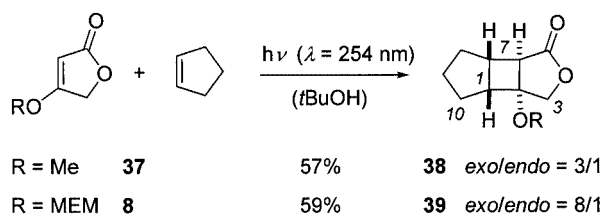
Scheme 11. Intermolecular cycloaddition of tetronates 8 and 37 and cyclopentene
