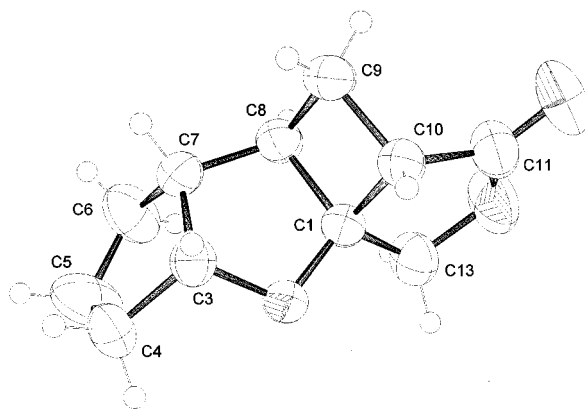
Figure 3. A molecule of 2,12-dioxatetracyclo[6.5.0.0 3,7 .0 1,10 ]tridecan-11-one ( 33a ) in the crystal
