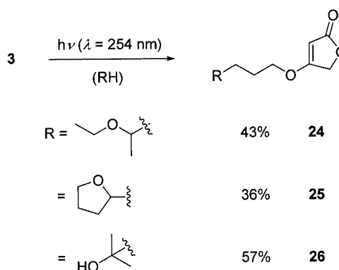
Scheme 6. Products obtained from solvent addition to allyl tetronate ( 3 ) upon irradiation
