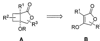
Scheme 1. Tetronates B as precursors of oxygen-containing heterocycles of general formula A
