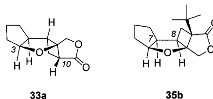
Figure 1. Stereochemical situation in the tetracyclic photocycloaddition products 33a ( cis-anti-cis -skeleton) and 35b ( cis-syn-cis -skeleton)
