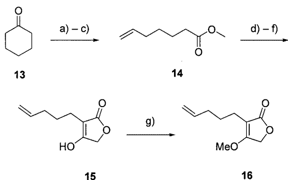
Scheme 3. Preparation of the C3-substituted methyl tetronate 16 from cyclohexanone ( 13 ): a) \text{Ac}_2\text{O} (neat), TSA, 60% b) \text{O}_3 , MeOH, DMS, then HOAc/THF/ \text{H}_2\text{O} (2:2:1), reflux, 48% c) \text{CH}_3\text{PPh}_3^+\text{I}^- , n\text{BuLi} in \text{Et}_2\text{O} , 46% d) TMS-Cl, LDA in THF e) \text{ClCH}_2\text{COCl} in THF f) DBU in toluene then 1 M HCl, 27% from 14 g) MeOH, \text{PPh}_3 , DIAD in THF, 92%
