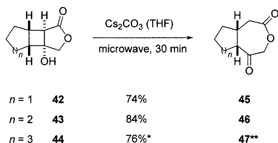
Scheme 13. Formation of oxepanediones 45–47 by retro aldol reaction of cycloaddition products 42–44 (* at 50% conversion based on recovered starting material; ** 1:1 diastereomeric mixture)
