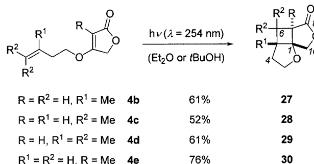
Scheme 7. Formation of substituted 2,9-dioxatricyclo[5.3.0]decanes 27–30 from tetronates 4b–4e
