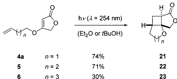
Scheme 5. Formation of strained tetrahydrofurans, tetrahydropyrans and oxepanes by intramolecular [2+2]-PCA of tetronates 4a , 5 and 6
