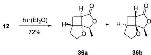
Scheme 10. Investigation of the facial diastereoselectivity in the cycloaddition of tetronate 12
