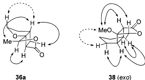
Figure 4. Structural assignments of photocycloaddition products 36a and exo - 38 on the basis of NOESY experiments
