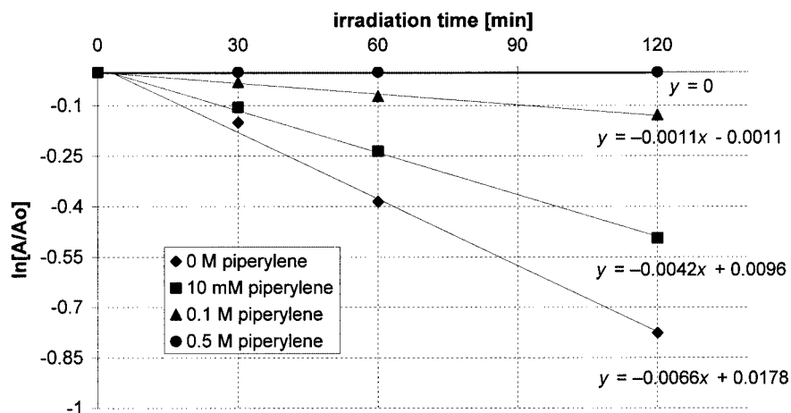
Figure 5. Quenching of the photocycloaddition of 4a to 21 by various amounts of piperlyene
