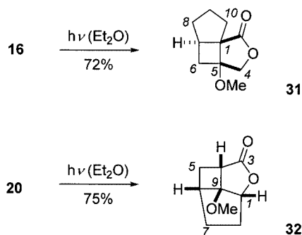
Scheme 8. Formation of tricyclic products 31 and 32 from C3-substituted tetronate 16 and C5-substituted tetronate 20
