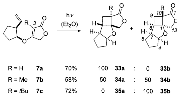
Scheme 9. Investigation of the facial diastereoselectivity in the cycloaddition of tetronates 7a – 7c
